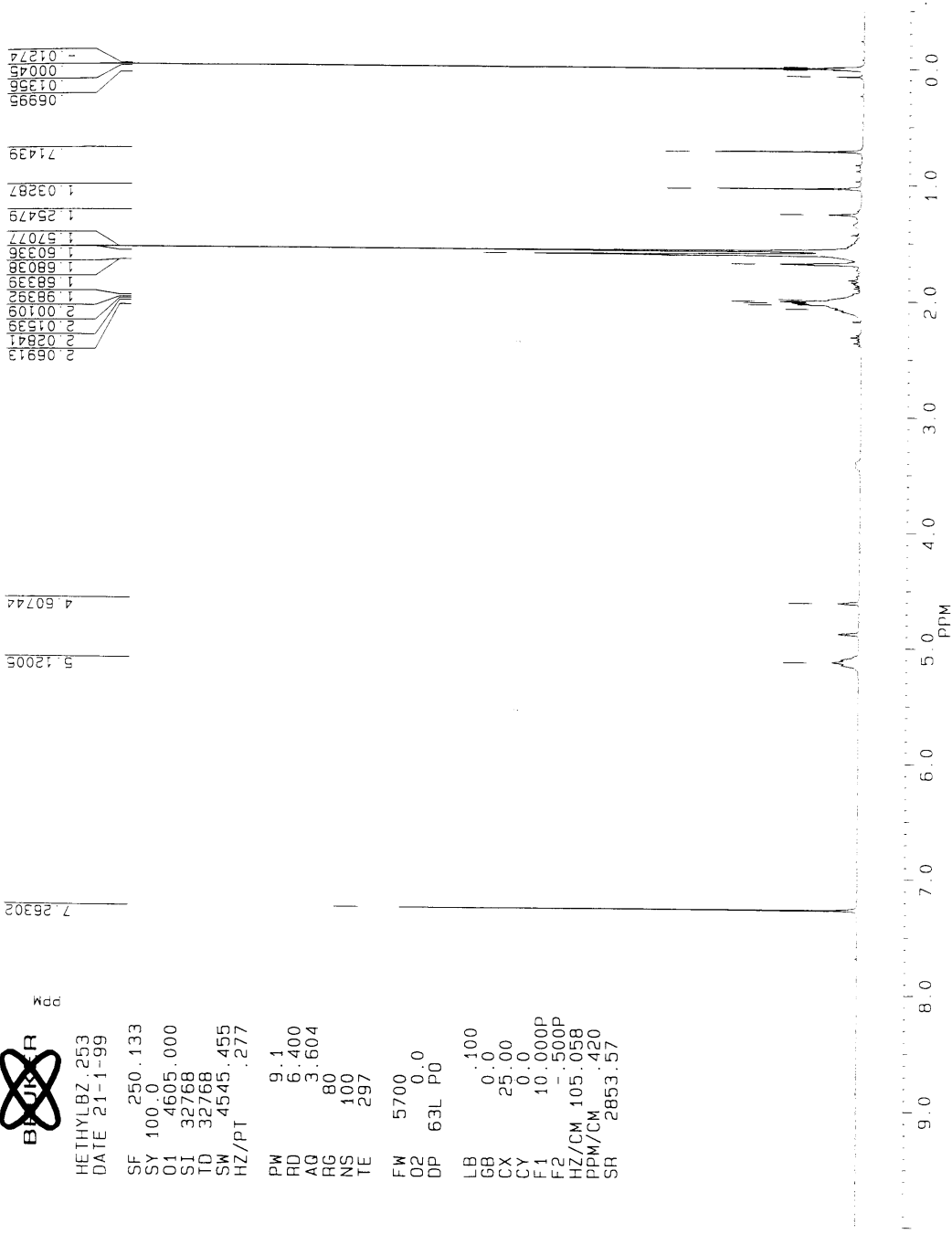
1 H-NMR spectrum of HPLC separated Achilleol A (Val454A mutant)
